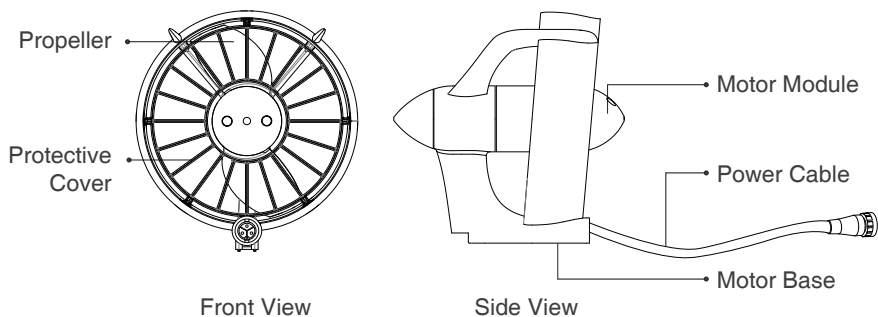
Figure 2-2 VAQUITA Motor
