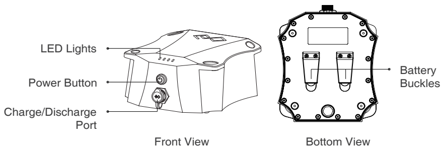
Figure 2-3 VAQUITA Battery
