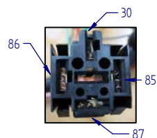
DETALLE RELES DE ARRANQUE / STARTER RELAY
