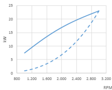
Vermogen (ISO 3046/1)
