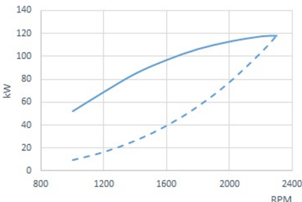
Power (ISO 3046/1)
