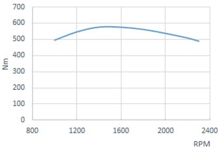
Crankshaft torque
