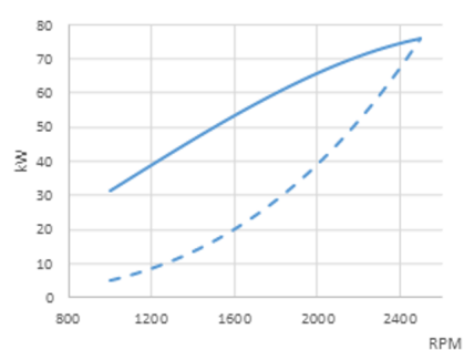
Vermogen (ISO 3046/1)
