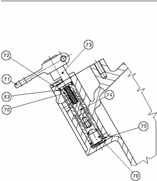
SELECTOR VALVE ASSEMBLY
