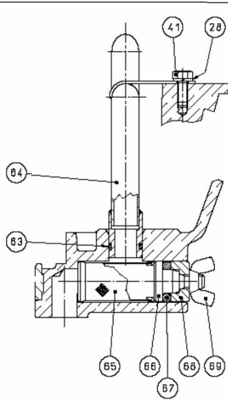
OIL FILTER ASSEMBLY
