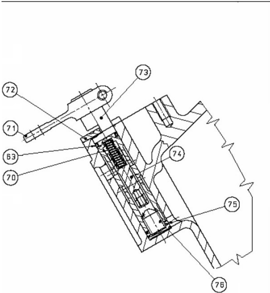
SELECTOR VALVE ASSEMBLY
